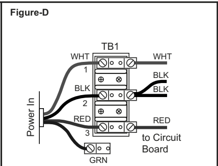
All US/Canada Denali/Tacoma Convertible Models: 120/240 VAC, 4-Wire Connection (60Hz)
