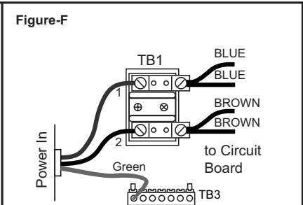
All Export Burlington/Denali/Tacoma Models: 230 VAC, 3-Wire (50Hz)
