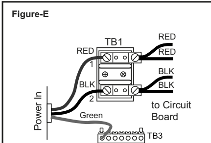
US/Canada Burlington Models: 240 VAC, 3-Wire Connection (60Hz)
