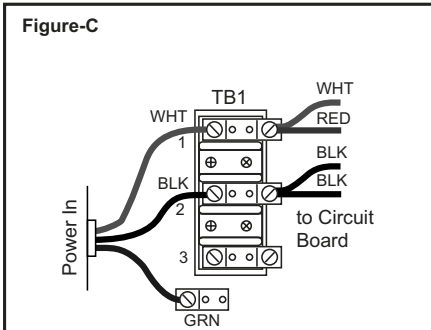
All US/Canada Denali/Tacoma Convertible Models: 120 VAC, 3-Wire Connection (60Hz)
